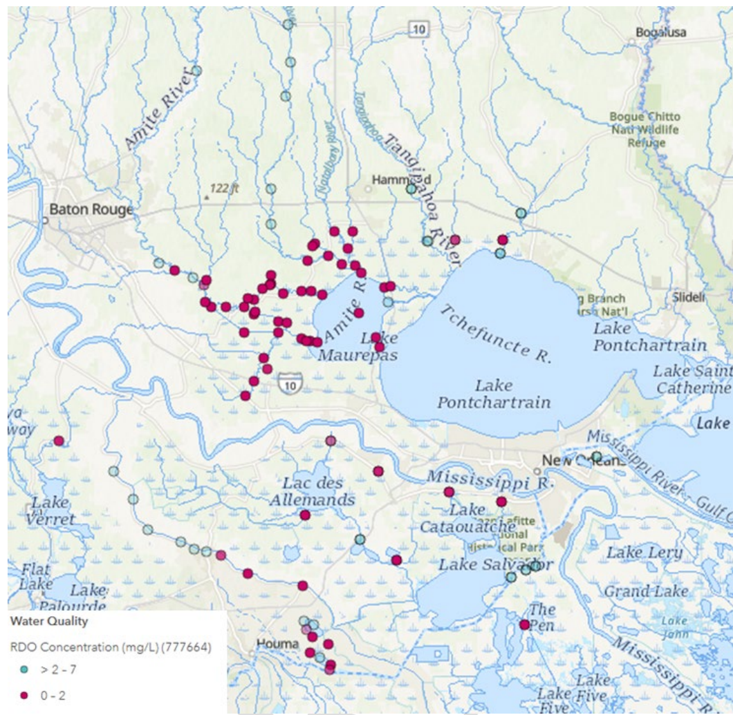
Figure 2. Dissolved oxygen following Hurricane measured between September 7 and September 16, 2021. Hypoxia ( < 2 \text{ mg/L} ) is in red, and transparency of points increases as oxygen concentration increases. Blue dots represent oxygen levels > 2 \text{ mg/L} , and increase in transparency as oxygen concentration increases.
