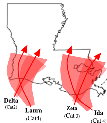
Figure 1. Tracks of Hurricanes Laura, Delta, Zeta, and Ida in 2020 and 2021
