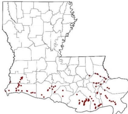
Figure 7. Location of coastal marinas, launches and other areas used in La Creel sampling in 2020 (n=131)
