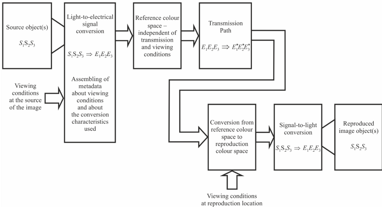
Block diagram of a potential adaptive system
