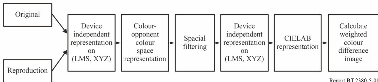
Flowchart of S-CIELAB
