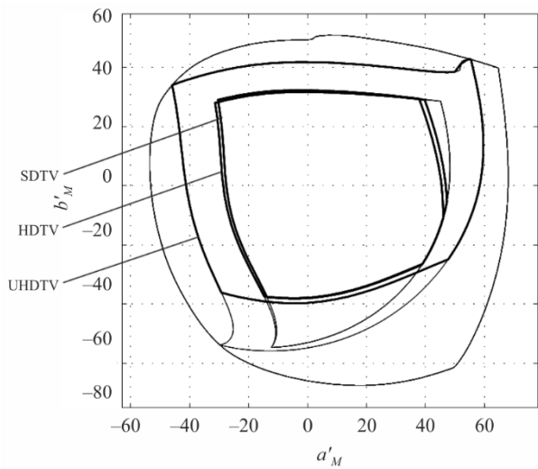
Colour gamuts of SDTV, HDTV and UHDTV systems for L_A = 50 \text{ cd/m}^2 in CAM02-UCS space
