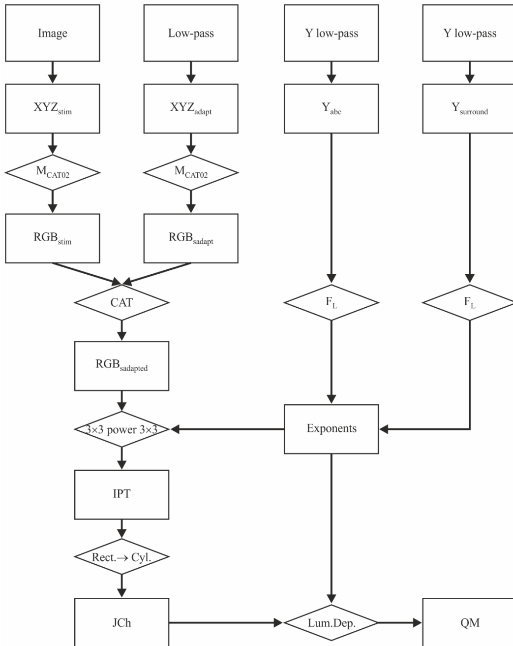
Flowchart of iCAM image appearance model
