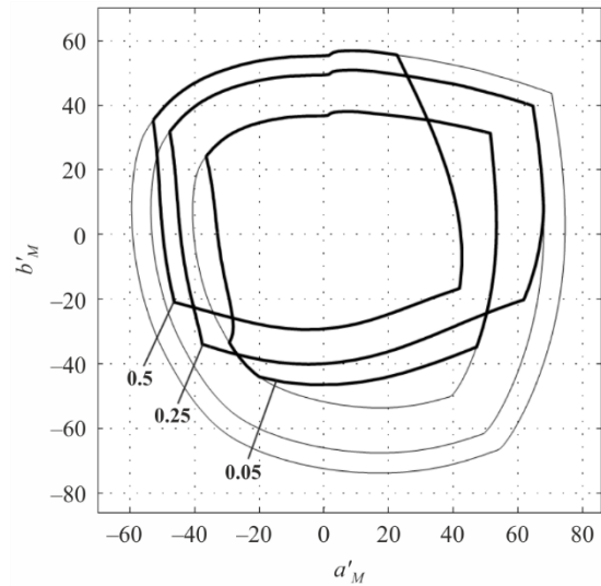
Colour gamut boundaries of DC system for L_A = 50 \text{ cd/m}^2 on the plane of a'_M, b'_M
