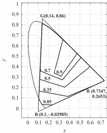
Colour gamut boundaries of DC system on the CIE-31 chromaticity diagram plane
