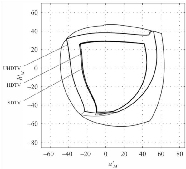
Colour gamuts of SDTV, HDTV and UHDTV systems for L_A = 50 \text{ cd/m}^2 in CAM02-UCS space
