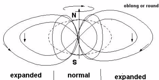
Figure 11. The atom as it spins.
