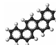
Hydrocarbons
