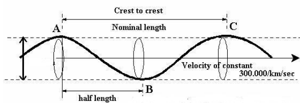
Figure 19. Light calculated for its 'relative' velocity.
